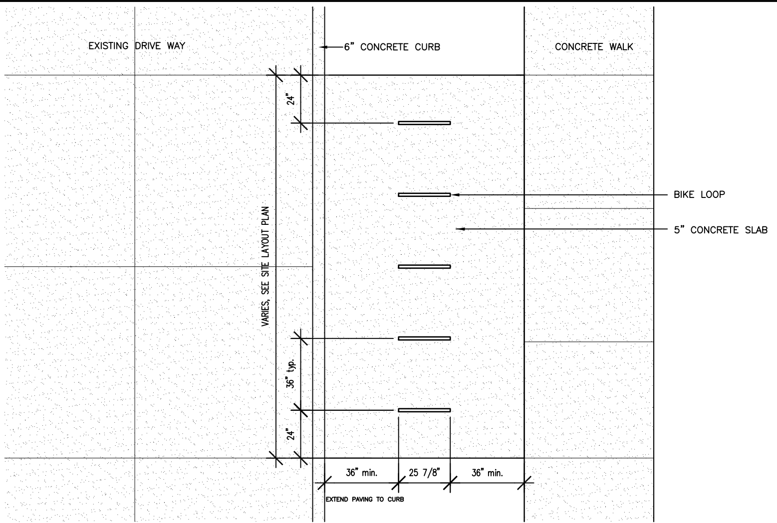
Bike Loop Plan Scale: 1/4"=1'-0"
