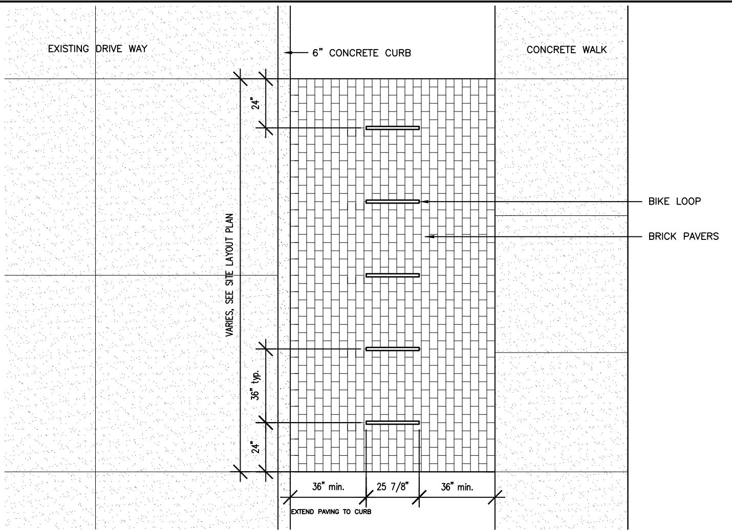
Bike Loop Plan Scale: 1/4"=1'-0"
