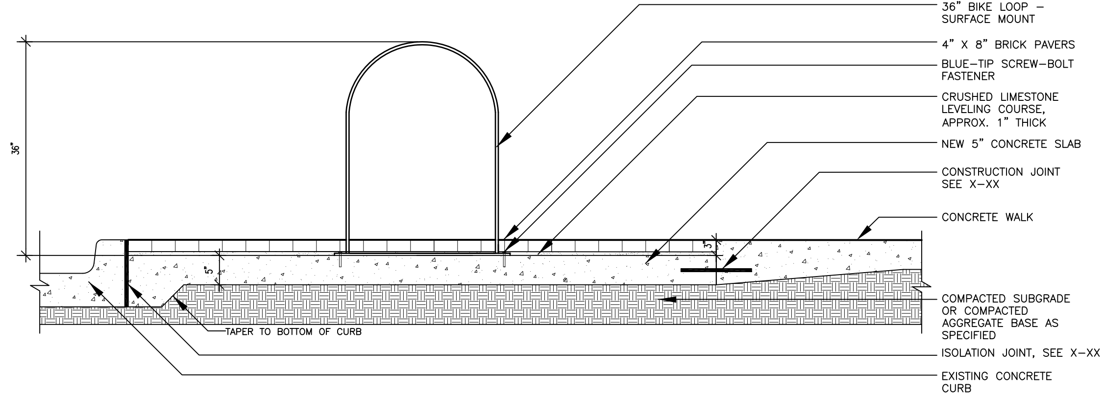
Bike Loop Section Scale: 3/4"=1'-0"
