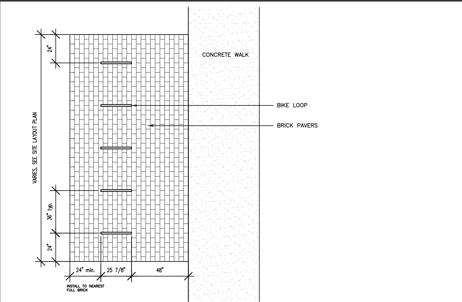
Bike Loop Plan Scale: 1/4"=1'-0"
