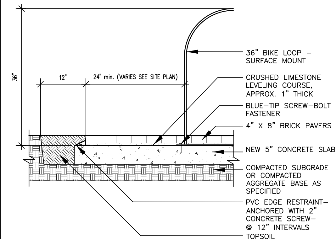
Bike Loop Section A Scale: 3/4"=1'-0"
