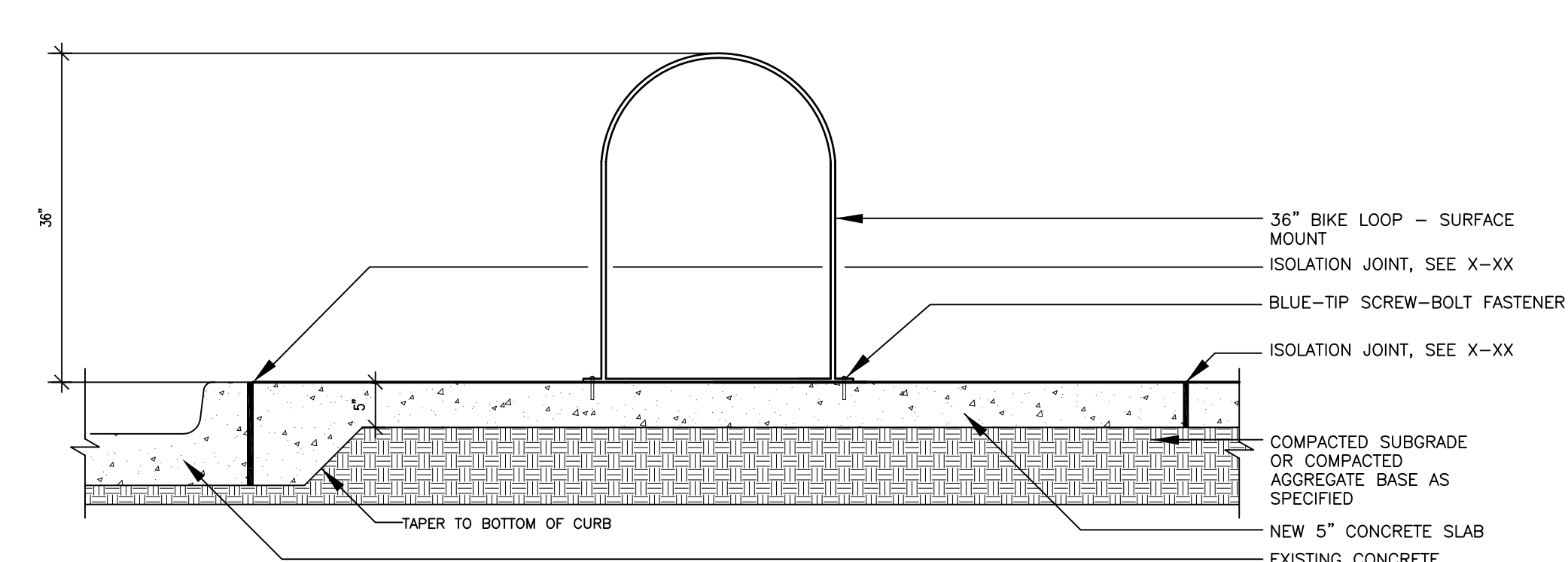
Bike Loop Section Scale: 3/4"=1'-0"
