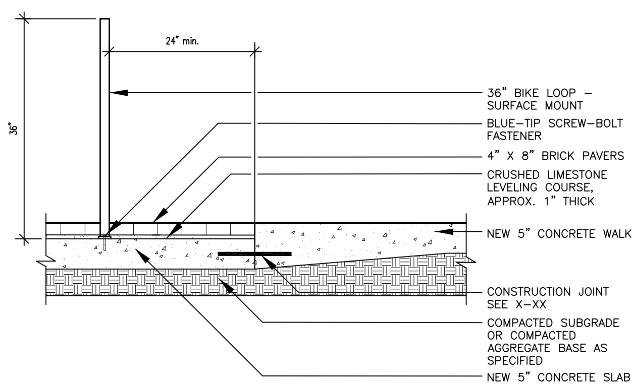
Bike Loop Section B Scale: 3/4"=1'-0"
