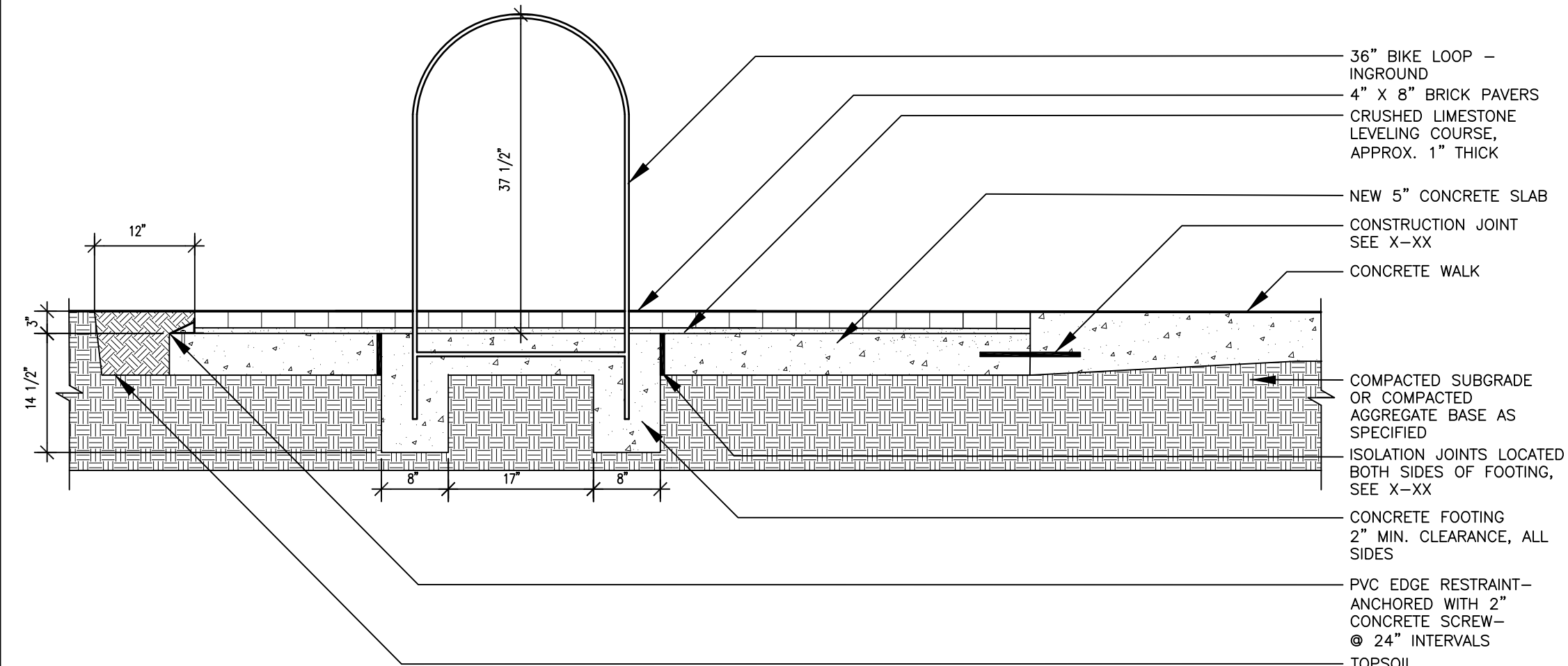
Bike Loop Section Scale: 3/4"=1'-0"
