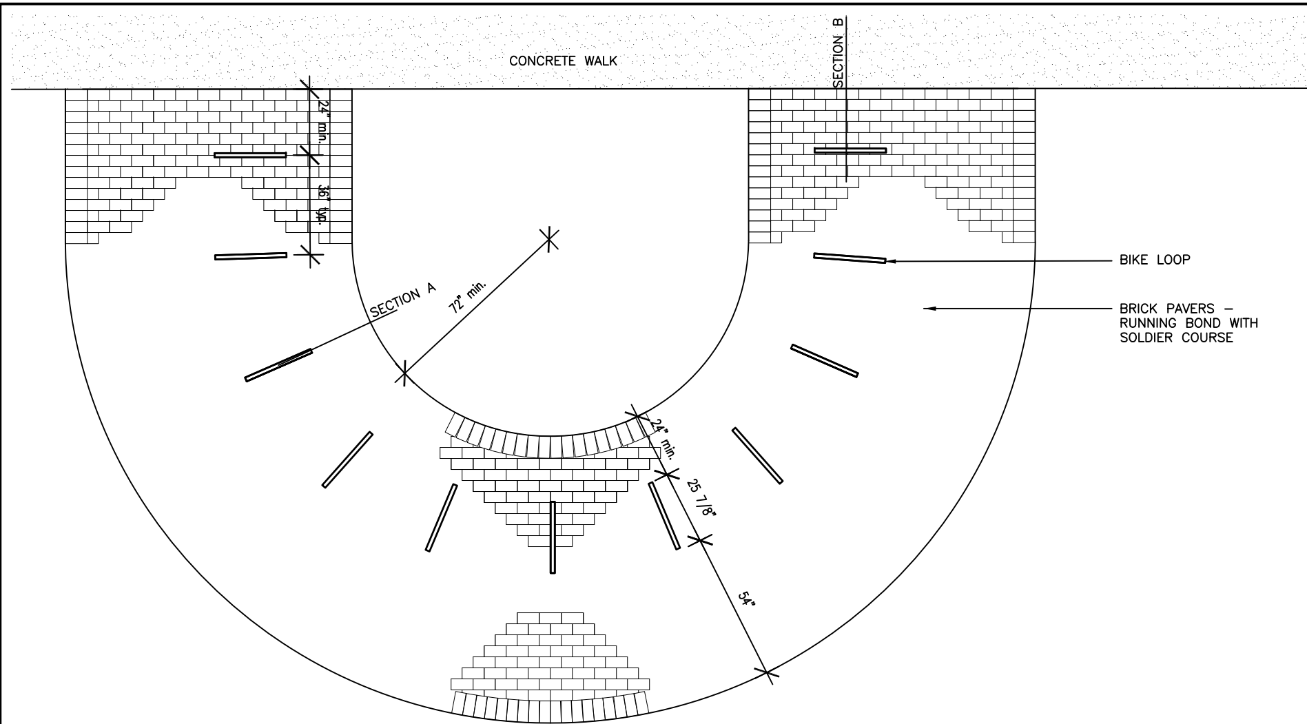
Bike Loop Plan Scale: 1/4"=1'-0"
