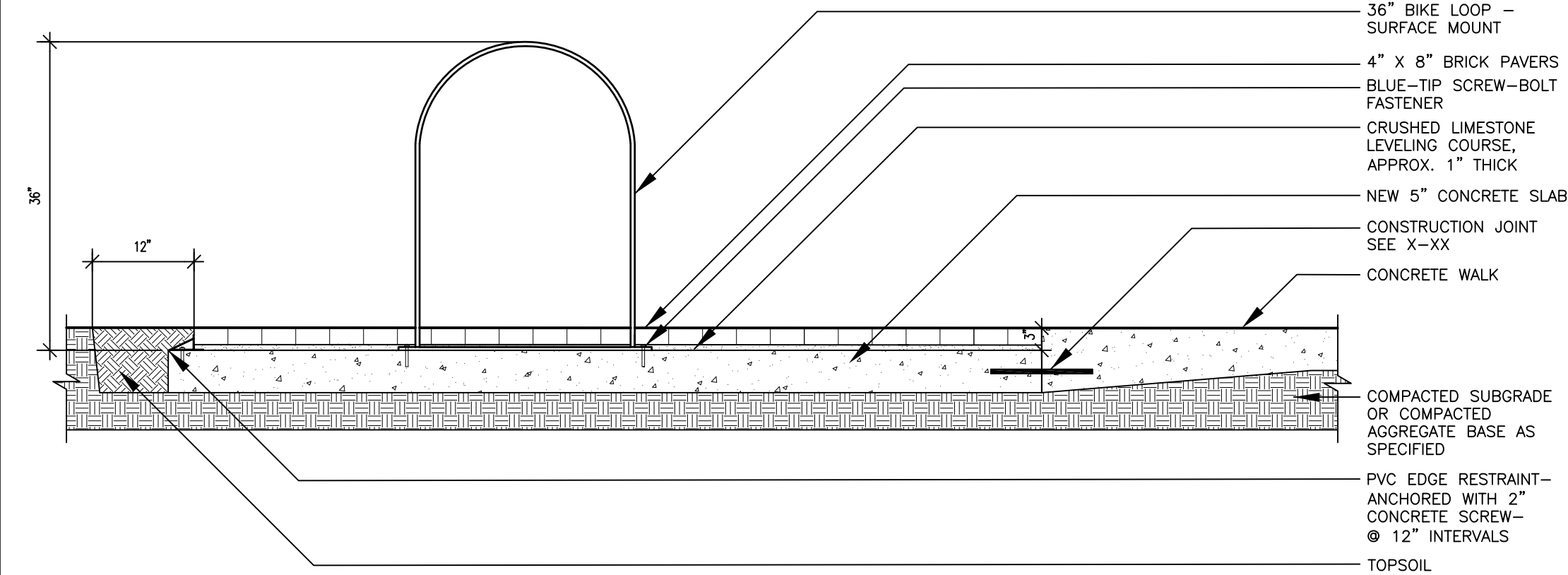
Bike Loop Section Scale: 3/4"=1'-0"
