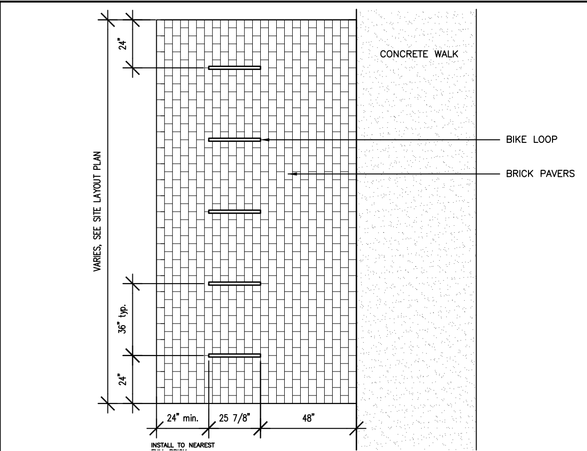
Bike Loop Plan Scale: 1/4"=1'-0"
